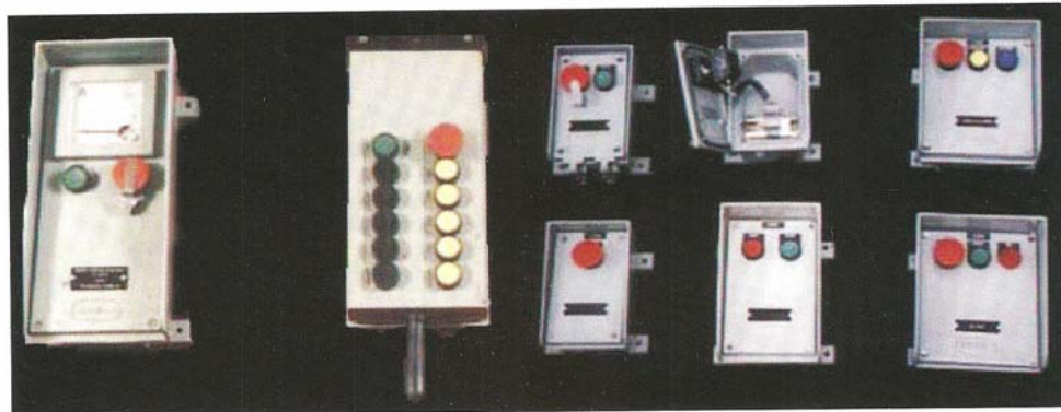
FRP & CAST ALUMINUM BOX : PUSH BUTTON WITH / WITHOUT CANOPY
